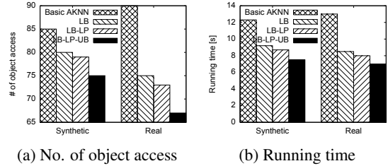
Figure 15: Effect of dataset
